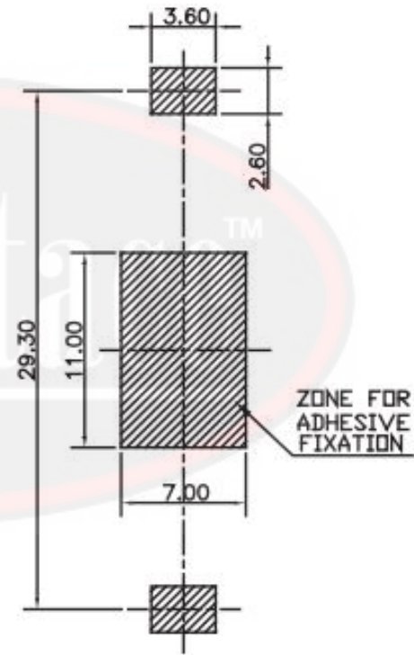
Recommended PCB Layout (PCB TOLERANCE \pm 0.05 )
