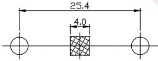
Recommended PCB Layout (PCB TOLERANCE \pm 0.05 )
