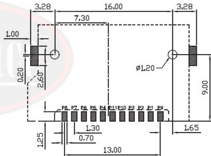
Recommended PCB Layout (PCB TOLERANCE ±0.05)
