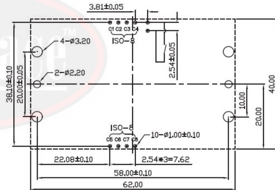
Recommended PCB Layout (PCB TOLERANCE ±0.05)
