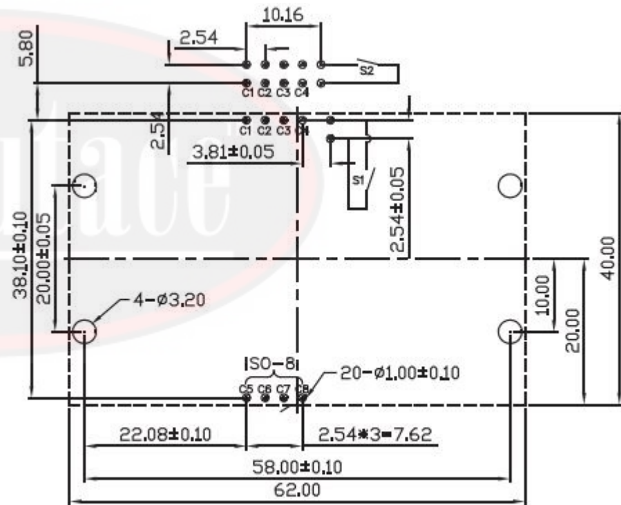
Recommended PCB Layout (PCB TOLERANCE ±0.05)
