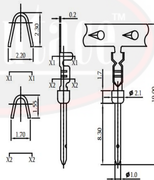
PART No.:32BR-S00M0002 1.0 Crimp Pin Male
