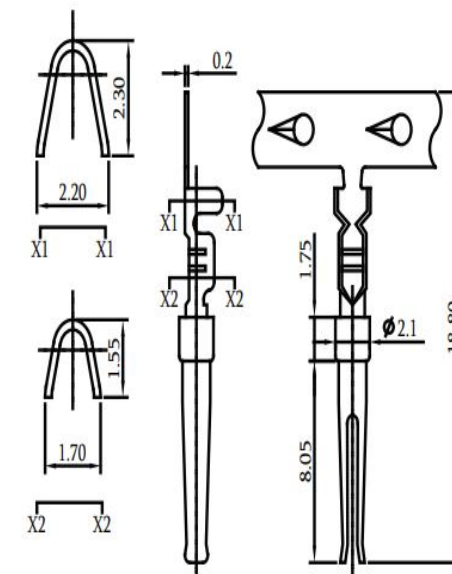
PART No.:32BR-S00F0002 1.0 Crimp Pin Female
