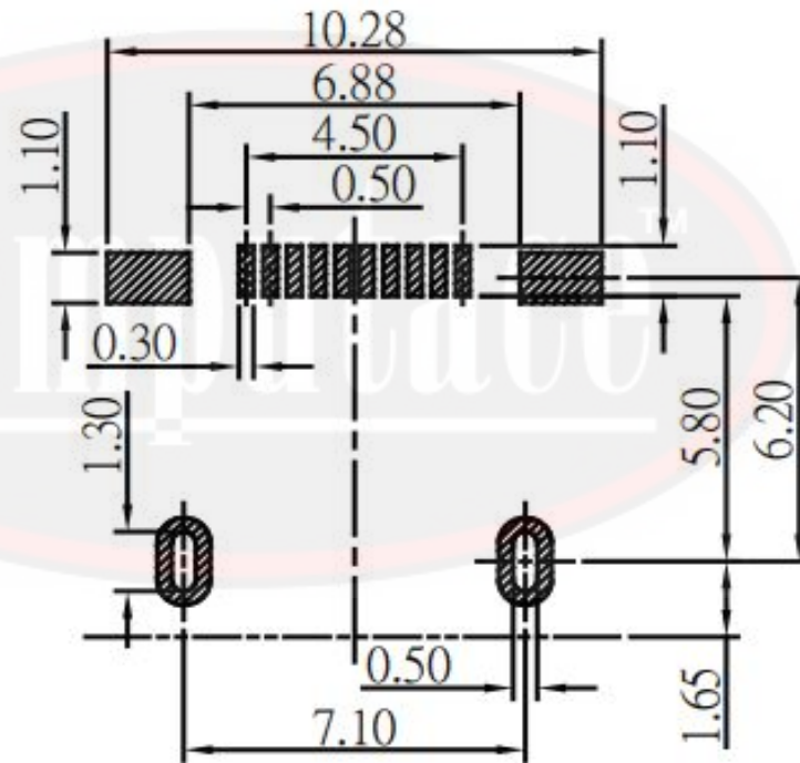
Recommended PCB Layout (PCB TOLERANCE \pm 0.05 )
