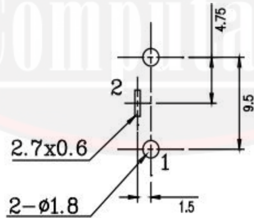
Recommended PCB Layout (PCB TOLERANCE \pm 0.05 )
