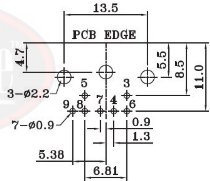
P.C.B. RECOMMEND LAYOUT BOTTOM VIEW
