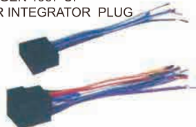
YY9549 CHRYSLER MOTORS 1978-90(12PIN) PLUGS INTO CAR HARNESS (POWER/4 SPEAKER)
