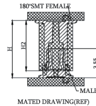
MATED DRAWING(REF)
